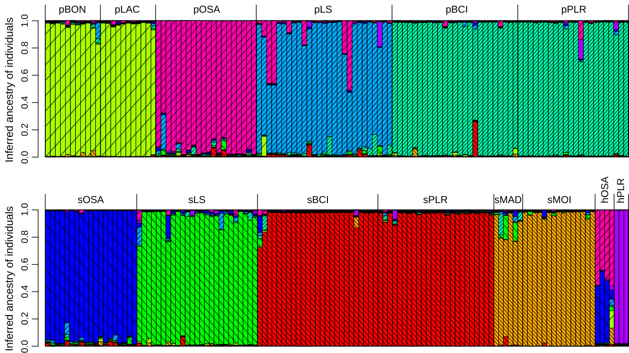
Fig. 2 Genetic structure of C. pulverulentus and C. scaber estimated by Bayesian assignment with K = 9 . Each vertical bar represents one individual, and the proportion of each colour within each bar corresponds to the proportion of the individual's genome assigned to each cluster. Individuals are ordered by population, and the codes correspond to the species name (p for C. pulverulentus , s for C. scaber and h for putative hybrids) followed by the population code (see Fig. 1 and Table 1). The two species are represented on separate lines for clarity, but all the samples have been analysed together.
